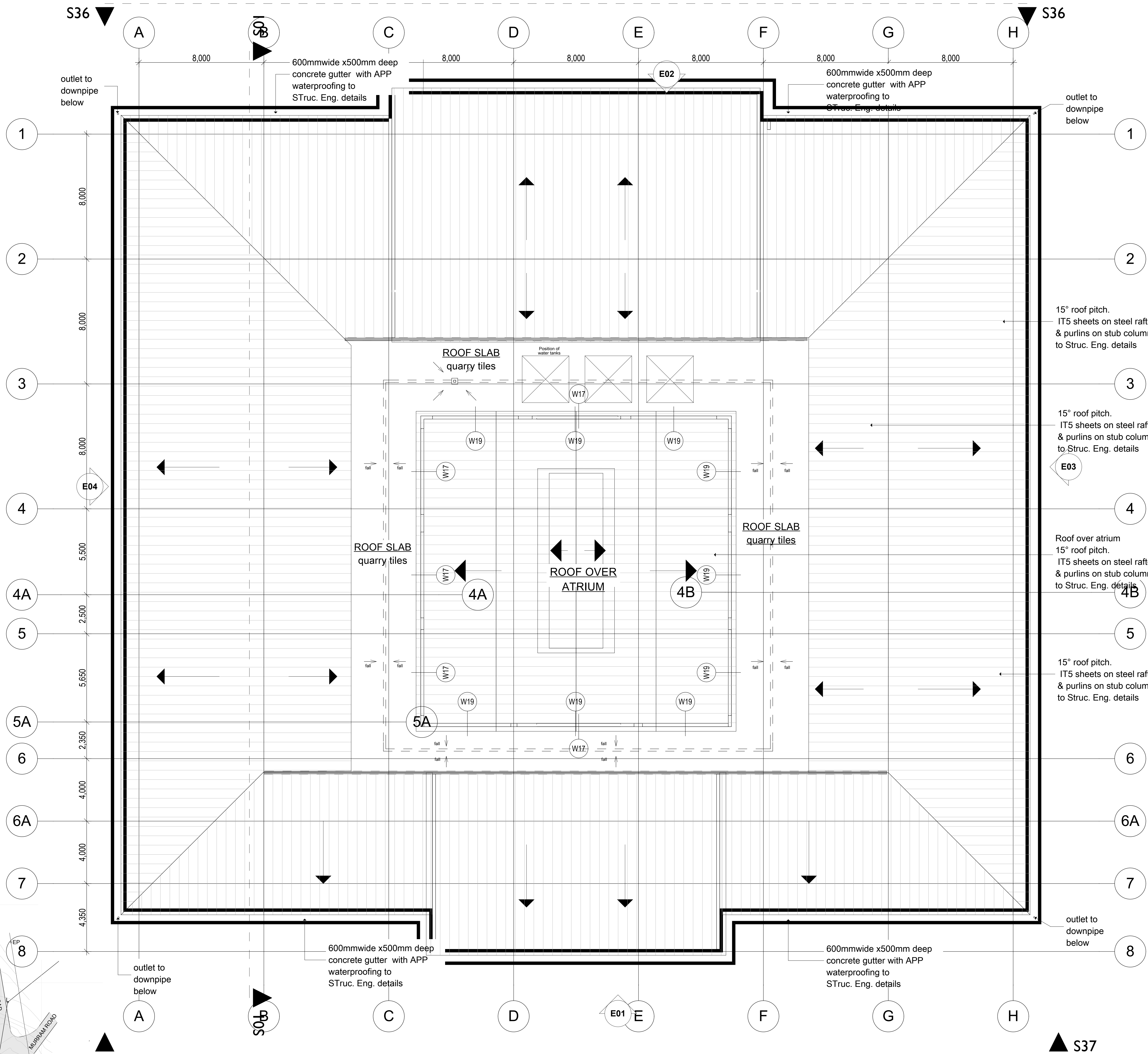
4. ROOF PLAN 1:100
